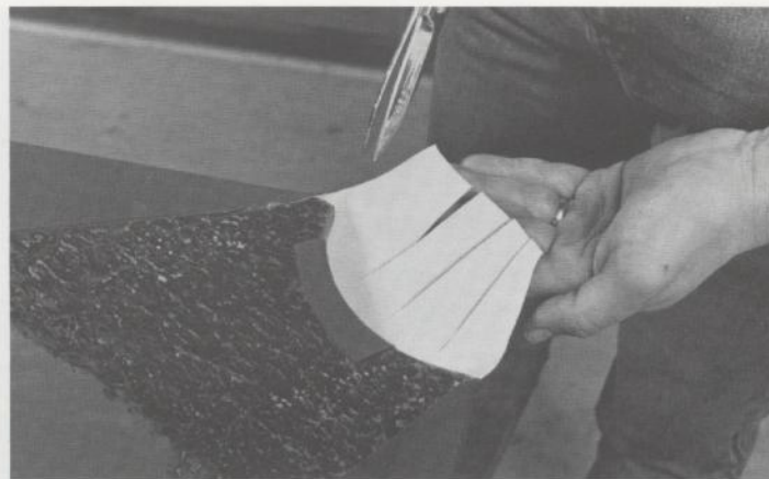
9 With a pair of scissors, cut the cloth on a radius at the end pockets and slice to within 1" of the slate. (Caution: Do not slice the cloth too close to the slate.)
