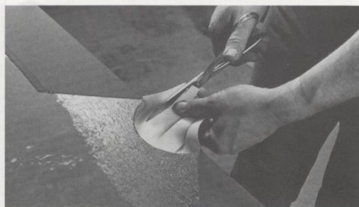
10 With a pair of scissors, cut a radius at the center pockets and slice the cloth to within 1" of the slate. (Caution: Do not slice the cloth too close to the slate.)
